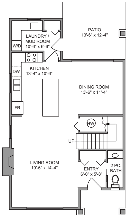
Main Floor 874 SQ FT
